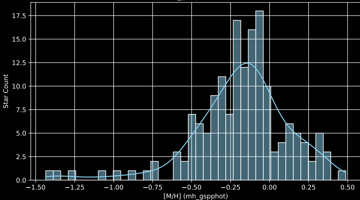
APOGEE DR17 Field: [048+41_MGA [M/H] (mh_gspphot) (n= 165)
