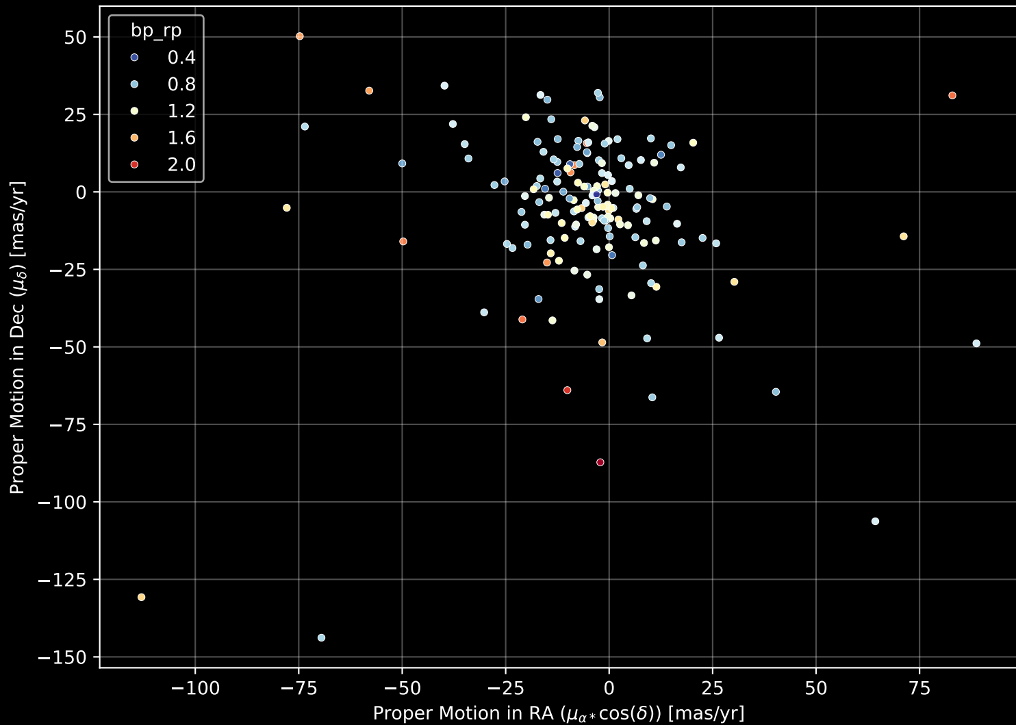
APOGEE DR17 Field: [048+41_MGA] Proper Motion Diagram (n= 166)
