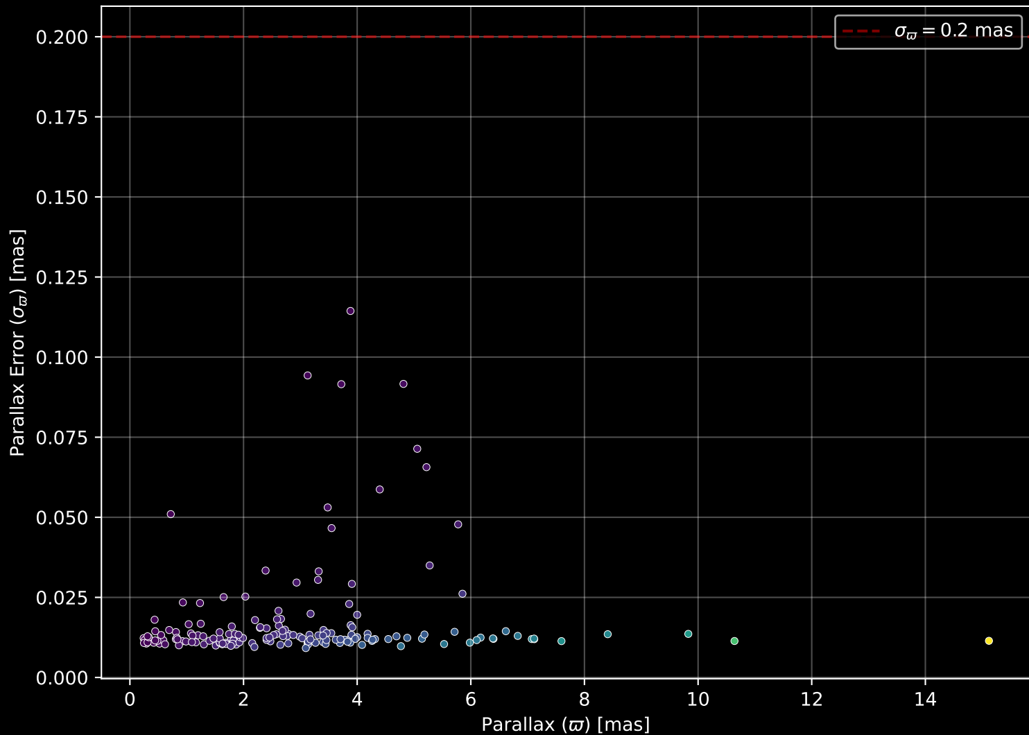
APOGEE DR17 Field: [048+41_MGA] Parallax Quality (n= 166)
