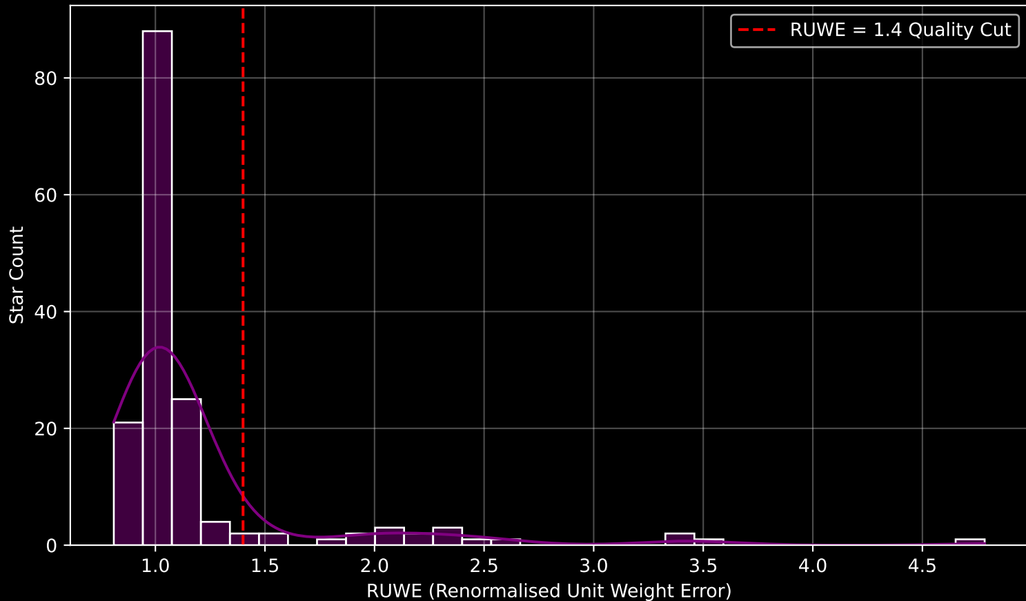
GAPOGEE DR17 Field [048+41_MGA] RUWE Distribution (n= 159)
