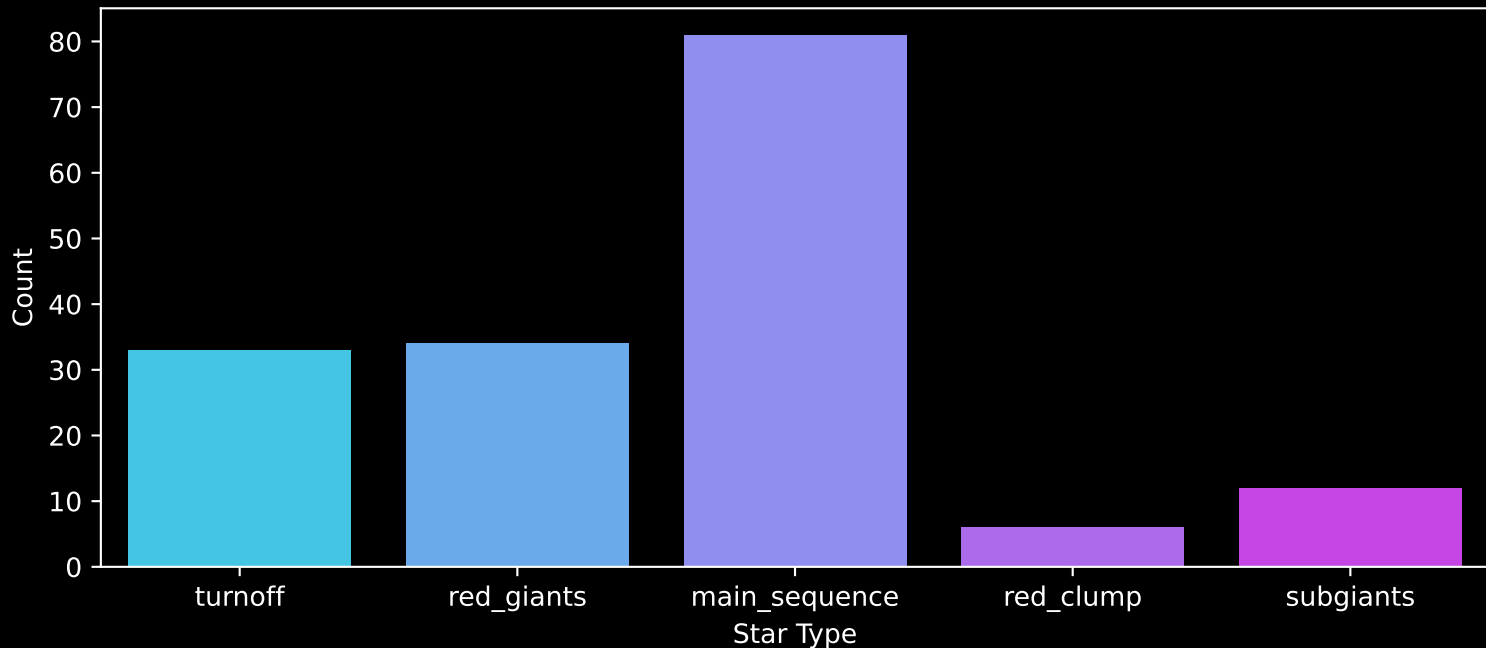
APOGEE DR17 Field: [048+41_MGA] Count plot of Star Type
